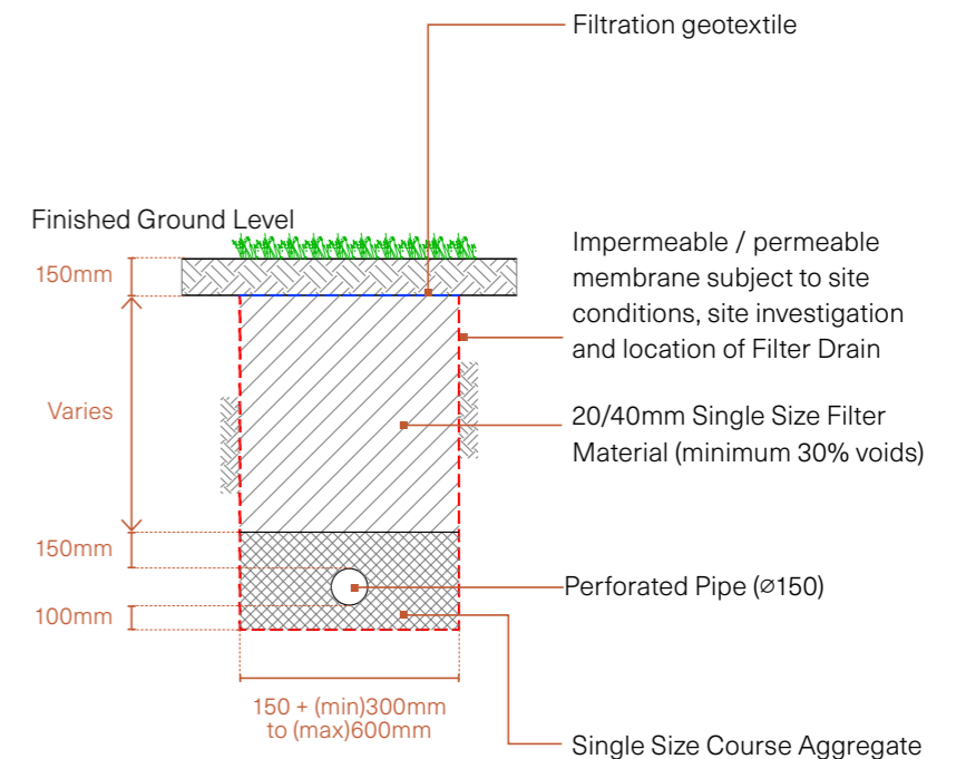
Figure 7: Typical Grassed Filter Drain Detail
