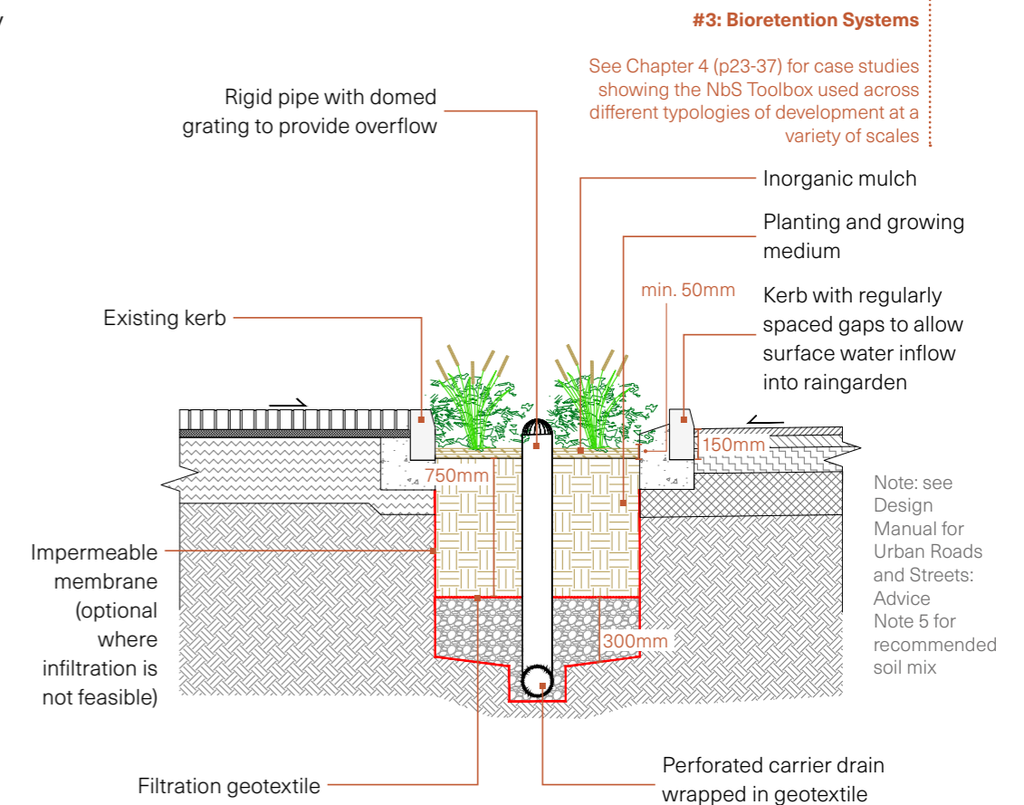
Figure 11: Typical Bioretention Raingarden Detail
