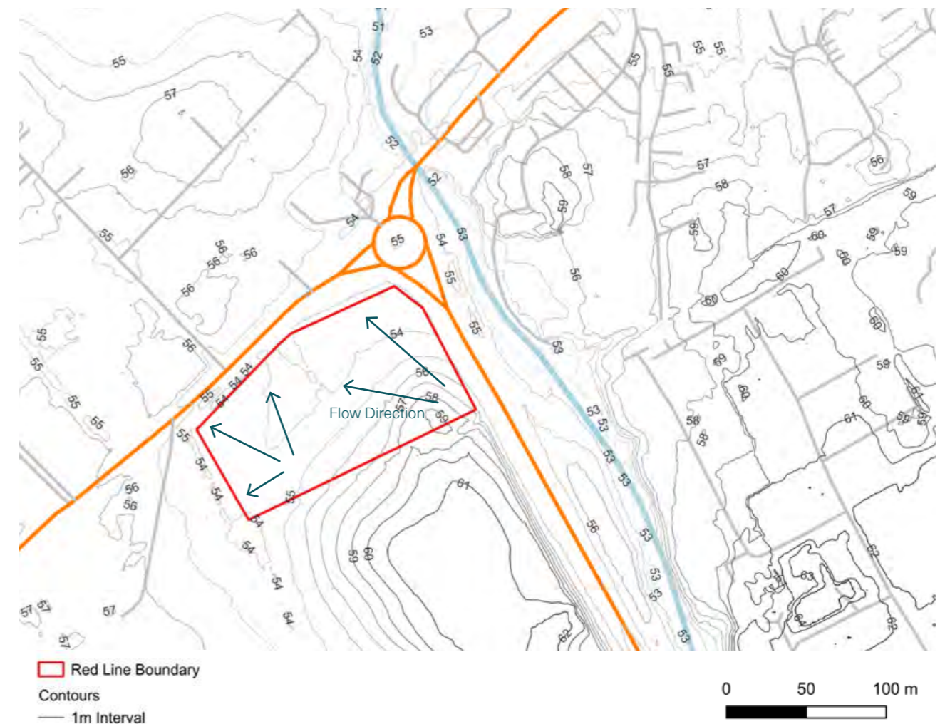
Figure C: Urban Residential Site – Topography
